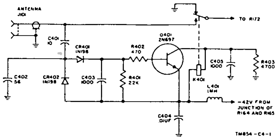
Figure 11.1 Rf input protective circuit.
