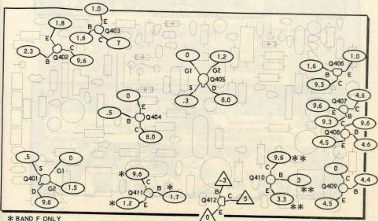
RECEIVER CIRCUIT BOARD (VIEWED FROM COMPONENT SIDE)
