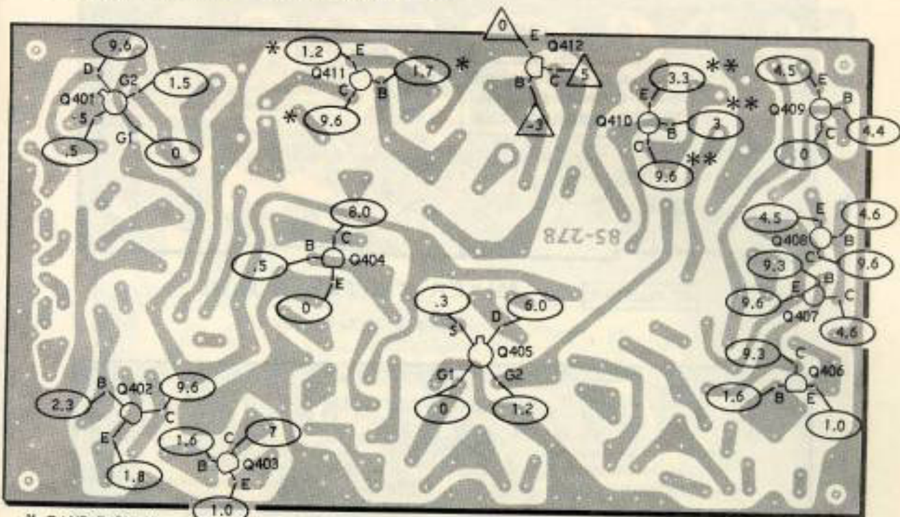
RECEIVER CIRCUIT BOARD (VIEWED FROM FOIL SIDE)
