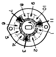
REAR OF WAFER LOOKING FROM REAR OF SWITCH
