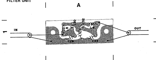
FILTER UNIT
