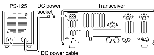
Connect to an AC outlet using the supplied AC cable.
