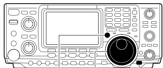
[XFC] Tuning dial [LOCK/SPCH]
