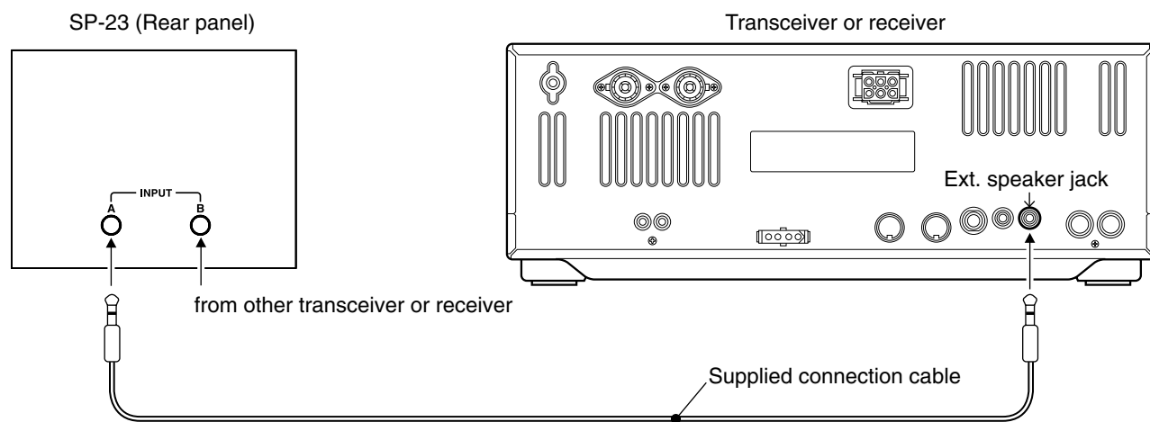
CONNECTION EXAMPLE
