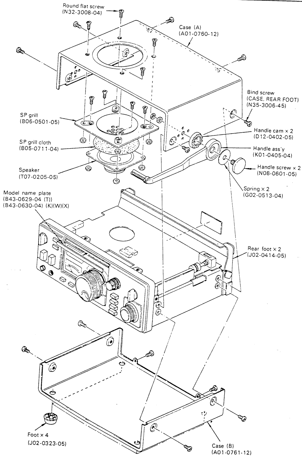
Fig. 3 Case disassembly
