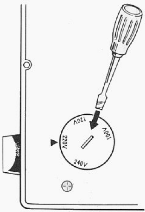
Fig. 2-2 AC Voltage Selection
