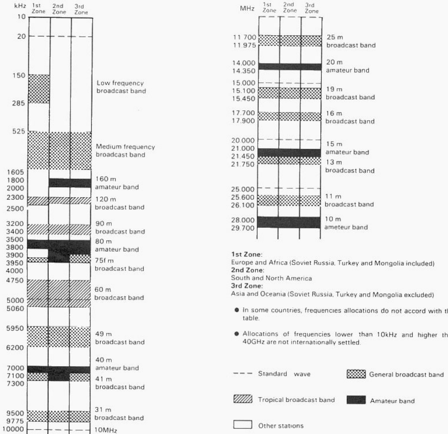
Fig. 6-2 Radio Frequency Allocation
