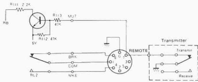
Fig. 5-1 Remote Terminal
