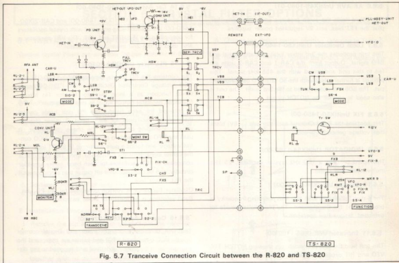
Fig. 5.7 Tranceive Connection Circuit between the R-820 and TS-820
