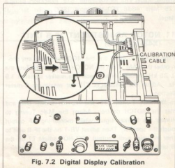
Fig. 7.2 Digital Display Calibration
