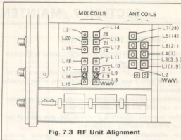
Fig. 7.3 RF Unit Alignment
