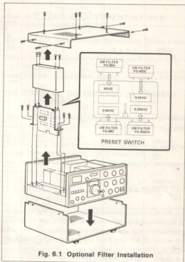
Fig. 6.1 Optional Filter Installation
