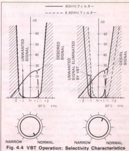
Fig. 4.4 VBT Operation: Selectivity Characteristics
