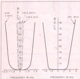
Fig. 4.2 IF Filters: Selectivity Characteristics
