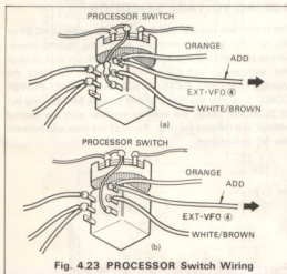
Fig. 4.23 PROCESSOR Switch Wiring
