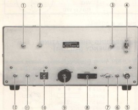
Fig. 3.2 Rear Panel
