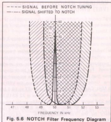
Fig. 5.6 NOTCH Filter Frequency Diagram
