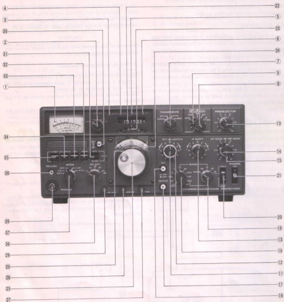
Fig. 3.1 Front Panel
