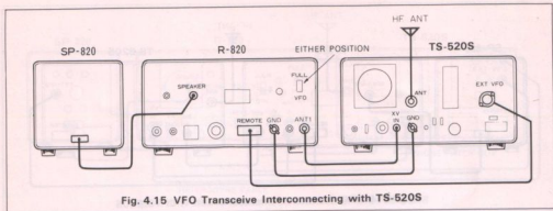
Fig. 4.15 VFO Transceiver Interconnecting with TS-520S
