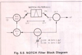
Fig. 5.5 NOTCH Filter Block Diagram
