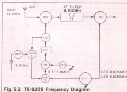
Fig. 5.2 TS-820S Frequency Diagram
