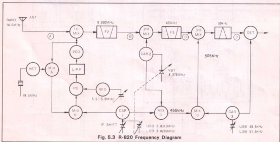
Fig. 5.3 R-820 Frequency Diagram
