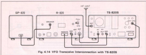
Fig. 4.14 VFO Transceiver Interconnection with TS-820S
