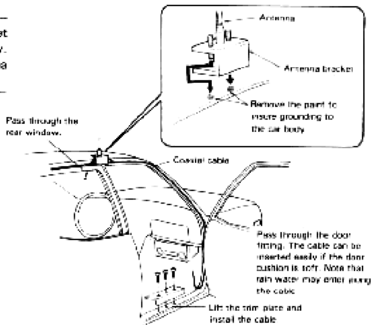
Coax. cable routing
