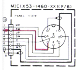
CONTROL UNIT (X53-1460-XX)(A/6)
