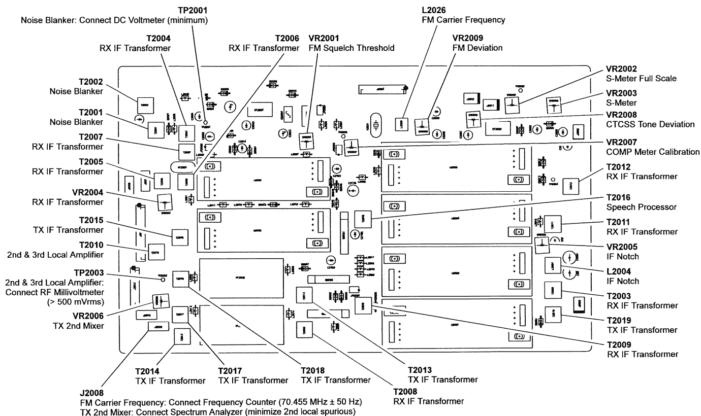
IF Unit Test & Alignment Points
