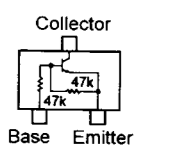
DTC144EU (26) (Q1040, 1041, 1042, 1043, 1044)
