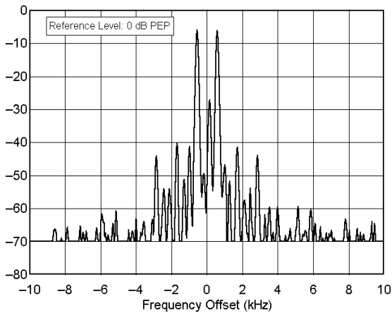
Yaesu FT-847 sn 8C020205 3.900 MHz, Transmit IMD, 100 W F:\SHARED\PROD_REV\TESTS\FT847\FT847160.TXT
