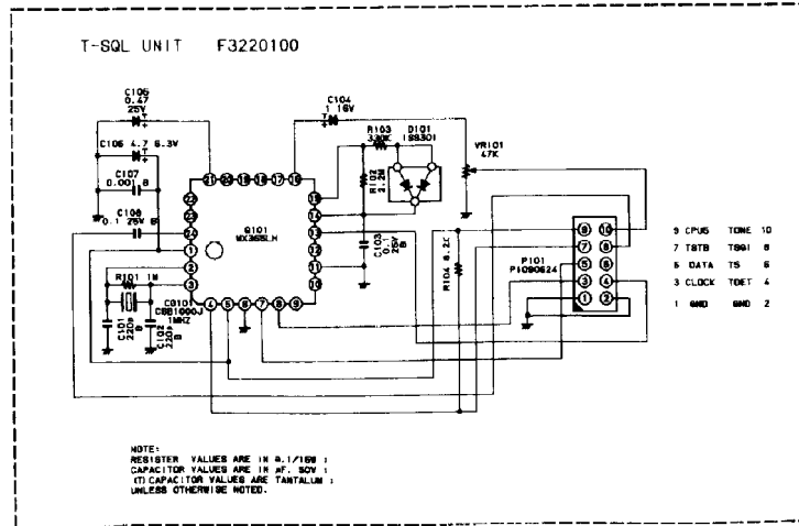
FTS-17A Circuit Diagram
